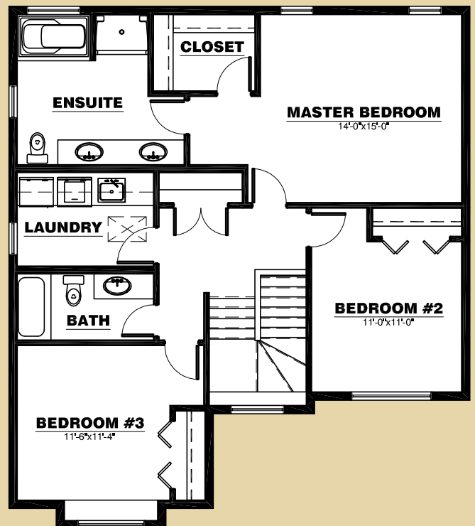
Second Floor | 1077 sq/ft
